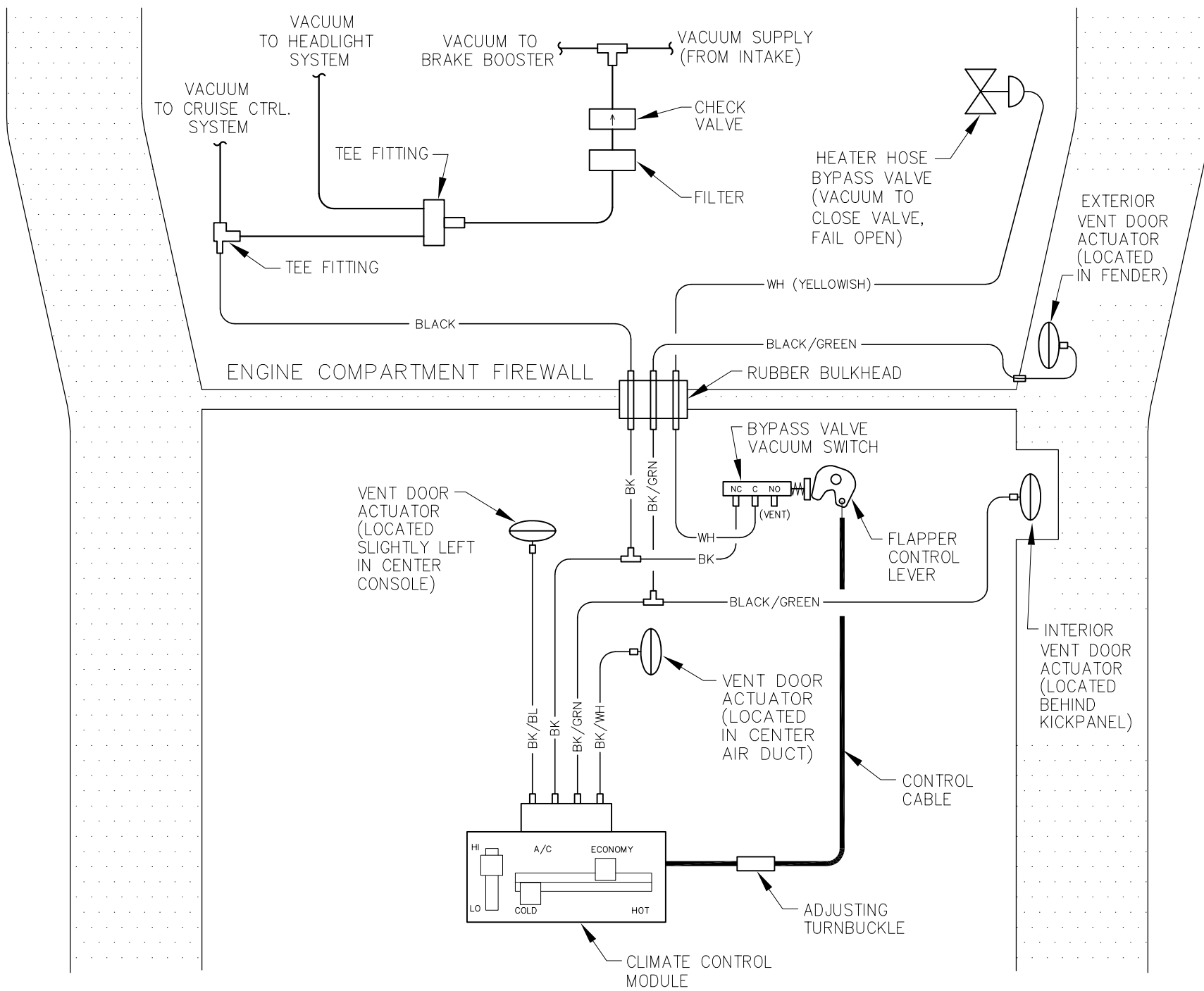
1977 CORVETTE CLIMATE CONTROL VACUUM DIAGRAM
